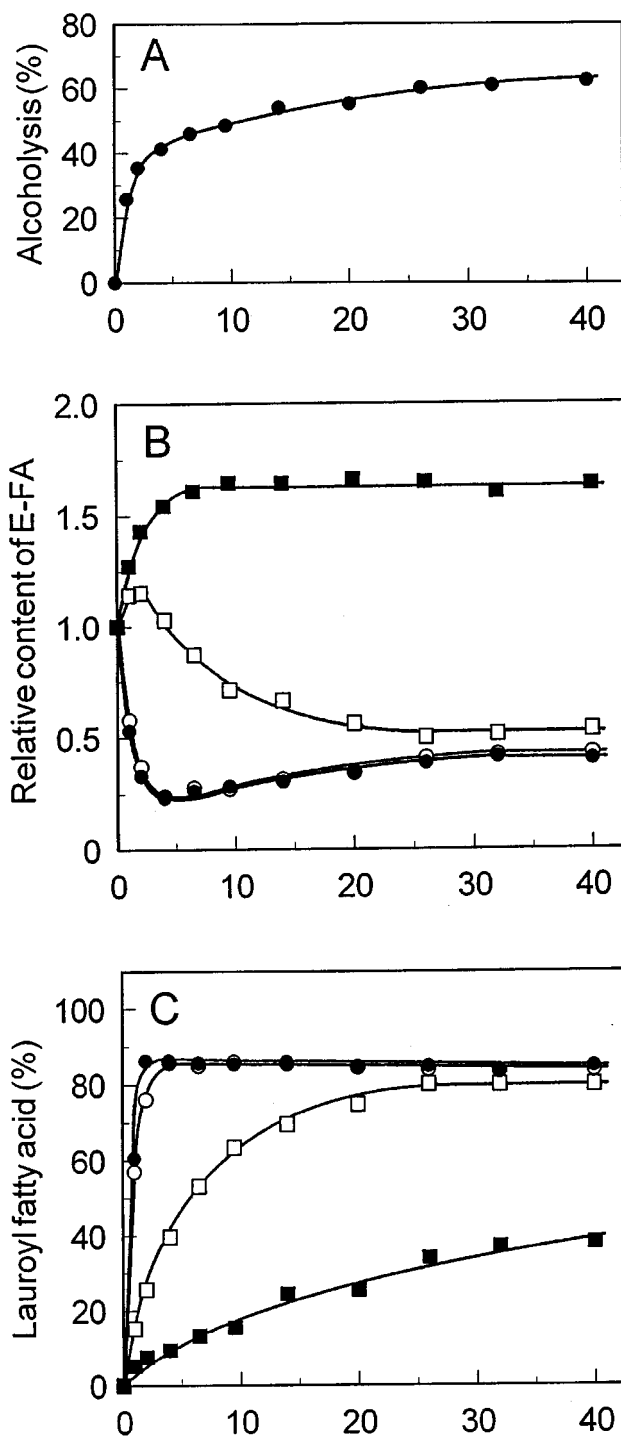
FIG. 2. Time course of the selective alcoholysis of E-tuna-45 with lauryl alcohol by immobilized Rhizomucor lipase. The reaction was conducted at 30°C with shaking in the mixture of 12 g E-tuna-45/lauryl alcohol (1:3, mol/mol) and 480 mg immobilized lipase. (A) Extent of alcoholysis. (B) E-FA content in the ethyl ester fraction. The content is expressed relative to the initial content: ethyl stearate, 5.2 mol%; ethyl oleate, 10.8 mol%; ethyl eicosapentaenoate, 12.5 mol%; ethyl docosahexaenoate, 44.9 mol%. (C) Conversion ratio of E-FA to lauryl ester. The amount of lauryl ester is expressed as a percentage of the initial E-FA content. Symbols in Figures B and C: ○, ester of palmitic acid; ●, ester of oleic acid; □, ester of eicosapentaenoic acid; ■, ester of docosahexaenoic acid. For abbreviations, see Figure 1.
