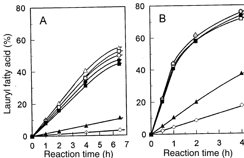
FIG. 4. Time course of the amount of lauryl ester generated in the alcoholysis of E-tuna-23 with immobilized Rhizopus delamar (A) or Rhizomucor miehei (B) lipase. The alcoholysis was conducted at 30°C with 4 wt% of the immobilized lipase. The amount of lauryl ester was expressed as a percentage of the initial content of the ethyl ester, 5.1 mol%); ●, lauryl palmitate (21.1 mol%); □, lauryl palmitoleate (5.8 mol%); ■, lauryl stearate (3.9 mol%); △, lauryl oleate (13.6 mol%); ▲, lauryl eicosapentaenoate (9.2 mol%); ◇, lauryl docosahexaenoate (22.7 mol%). For abbreviation, see Figure 1.
